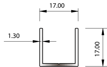
SECTION No. 31017 0.170 kg/m P = 98.88
