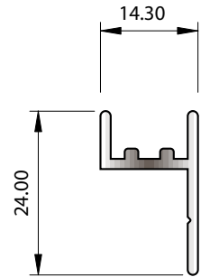
SECTION No. J031 0.191 kg/m P = 94
