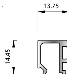
SECTION No. 5653 0.166 kg/m P = 97.50
