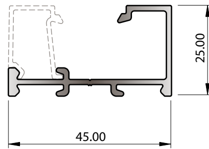
SECTION No. Z662 0.442 kg/m P = 207.66
