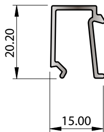
SECTION No. Z661 0.184 kg/m P = 114.92
