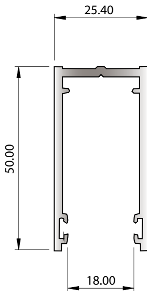
SECTION No. 33604 0.742 kg/m P = 275.99
