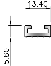
SECTION No. 38959 0.115 kg/m P = 100
