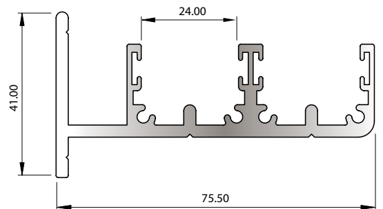
SECTION No. 34689 1.521 kg/m P = 453.62 LENGTH = 4.6m
