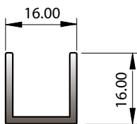
SECTION No. 5979 0.194 kg/m P = 92.80
