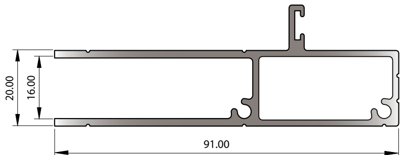
SECTION No. 33630 1.200 kg/m P = 369.10
