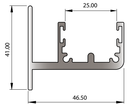
SECTION No. 33628 0.936 kg/m P = 295.94 LENGTH = 4.6m
