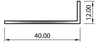
SECTION No. 7084 0.205 kg/m P = 104
