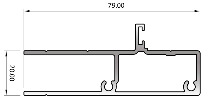
SECTION No. J007D 1.022 kg/m P = 320.58
