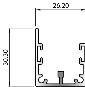
SECTION No. 30973 0.421 kg/m P = 210.39
