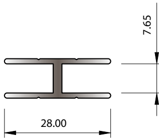
SECTION No. X574 0.249 kg/m P = 126.32
