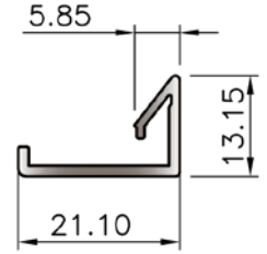
SECTION No. 36405 0.154 kg/m P = 87.09
