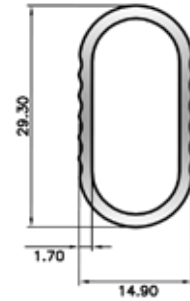
SECTION No. 36157 0.310 kg/m P = 76.58
