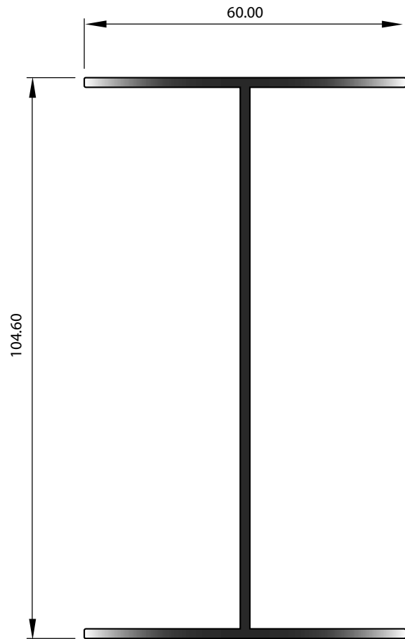
SECTION No. G902 1.078 kg/m P = 445.57
