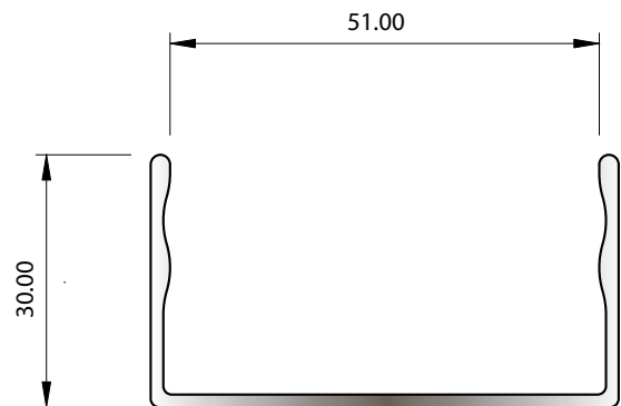
SECTION No. 8570 0.501 kg/m P = 226.56
