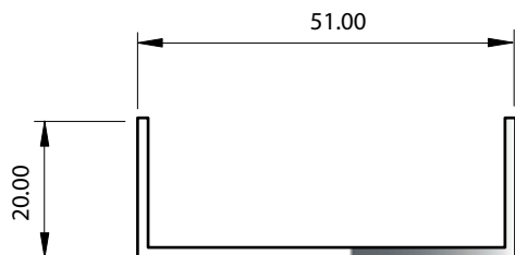
SECTION No. 6330 0.370 kg/m P = 185
