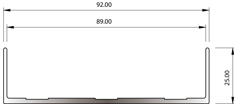
SECTION No. Z381
