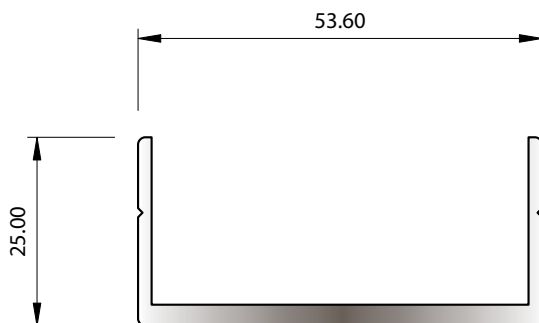
SECTION No. 7414 0.620 kg/m P = 200.87
