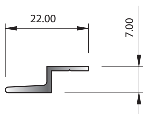
SECTION No. K804 0.106 kg/m P = 56.70
