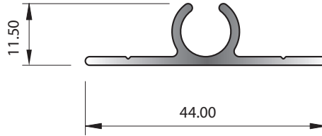
SECTION No. 8955 0.279 kg/m P = 129.99
