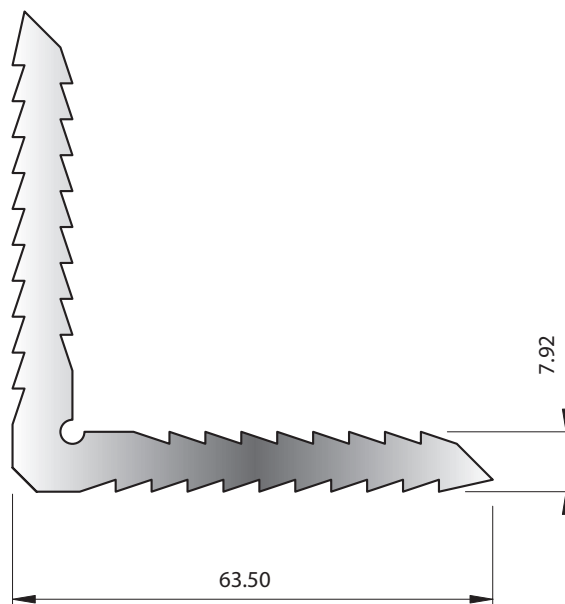
SECTION No. 1754 1.999 kg/m P = 312
