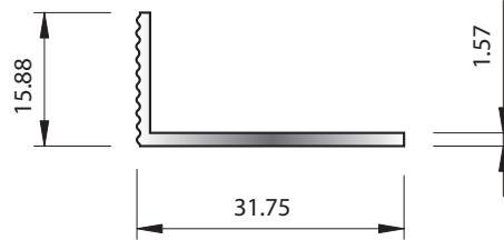
SECTION No. 2089 0.187 kg/m P = 97
