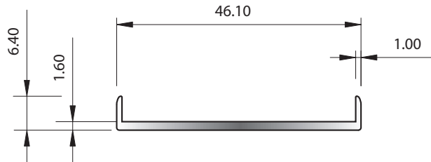
SECTION No. K768* 0.224 kg/m P = 113.08
