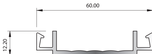
SECTION No. J030 0.496 kg/m P = 199
