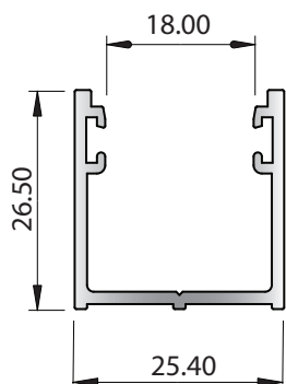
SECTION No. 33602 0.353 kg/m P = 178.41
