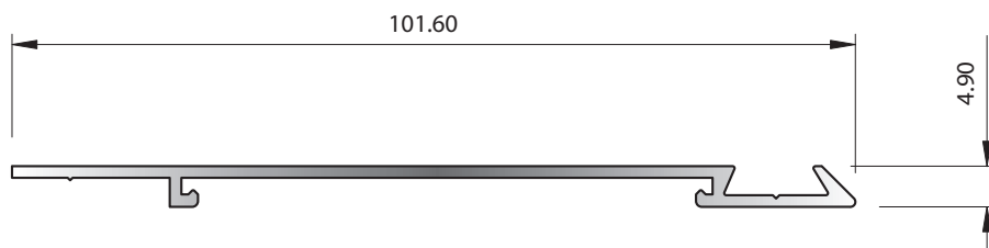
SECTION No. J395* 0.452 kg/m P = 236.40
