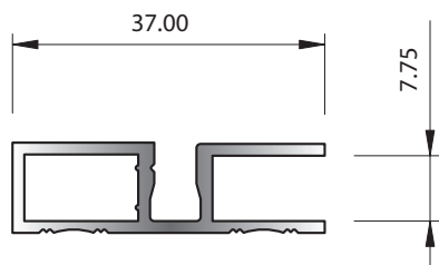
SECTION No. 5663 ACCEPTS STAKING ANGLE 6180 0.351 kg/m P = 143.50
