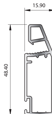
SECTION No. 31966 0.515 kg/m P = 156.98
