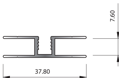
SECTION No. 6488 0.260 kg/m P = 171.55
