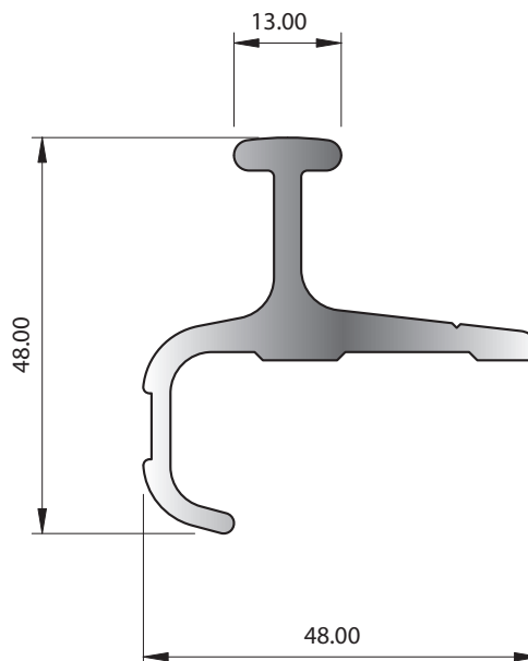
SECTION No. 7509 1.046 kg/m P = 210.62
