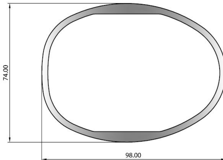
SECTION No. 35010 2.629 kg/m Ext. P = 276.63
