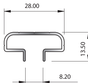
SECTION No. K080 0.176 kg/m P = 134.94
