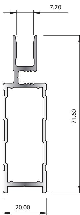
SECTION No. Z340* 0.751 kg/m P = 240.51
