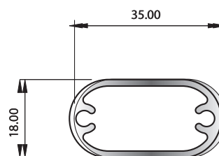
SECTION No. X534 0.430 kg/m P = 90.55
