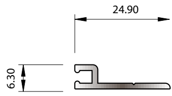
SECTION No. X389 0.139 kg/m P = 71.64
