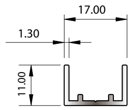
SECTION No. 31018 0.139 kg/m P = 81.16
