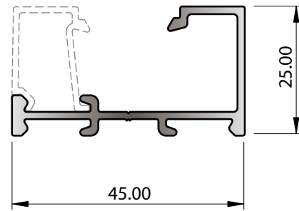
SECTION No. Z662 0.442 kg/m P = 207.66
