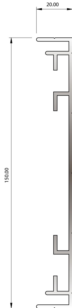
SECTION No. X540 1.418 kg/m P = 528.89
