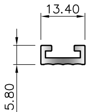
SECTION No. 38959 0.115 kg/m P = 100
