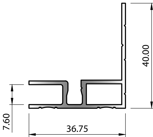
SECTION No. 6179 0.462 kg/m Ext. P = 200.42
