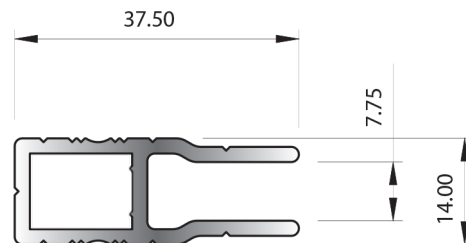
SECTION No. G253 0.500 kg/m P = 194.49
