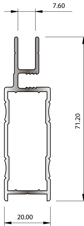
SECTION No. Z785 ACCEPTS STAKING ANGLE 6868K 0.748 kg/m P = 240.25
