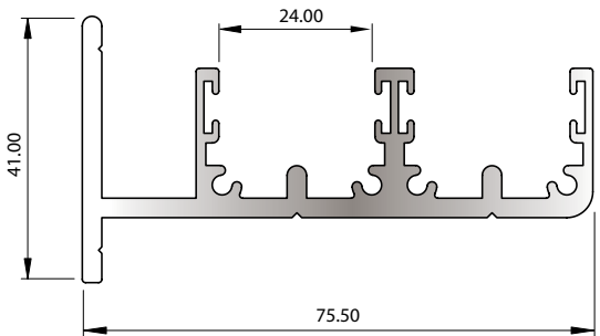
SECTION No. 34689 1.521 kg/m P = 453.62 LENGTH = 4.6m
