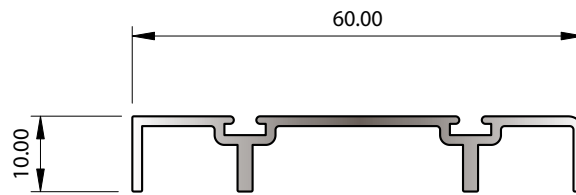
SECTION No. 33956 0.382 kg/m P = 205.55
