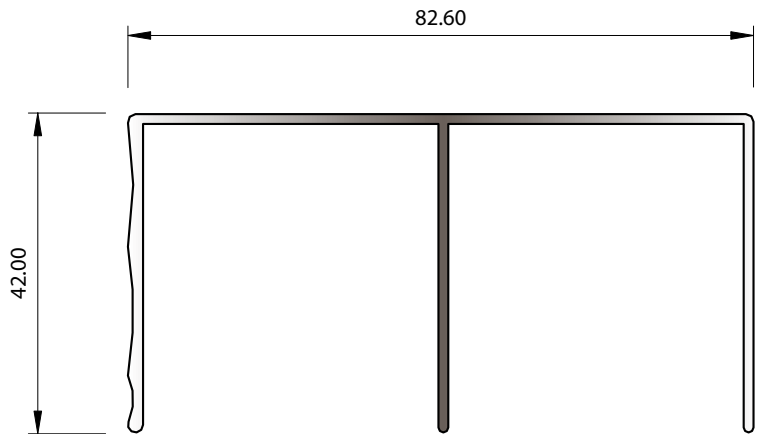
SECTION No. N924 0.745 kg/m P = 409.90
