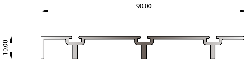
SECTION No. 33957 0.543 kg/m P = 290.37
