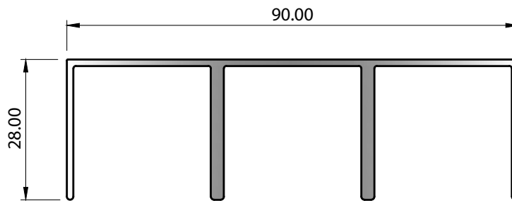
SECTION No. 33954 0.880 kg/m P = 392.51
