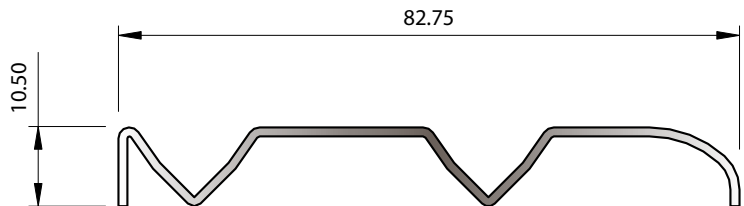
SECTION No. N923 0.370 kg/m P = 230.10
