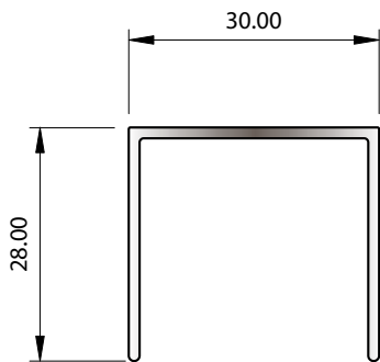
SECTION No. 33952 0.293 kg/m P = 167.68
