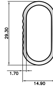
SECTION No. 36157 0.310 kg/m P = 76.58
