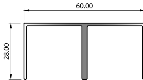
SECTION No. 33953 0.587 kg/m P = 280.10
