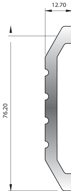
SECTION No. 0732 1.154 kg/m P = 181
