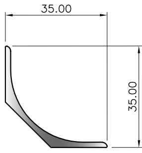
SECTION No. 7789 0.360 kg/m P = 118.32
