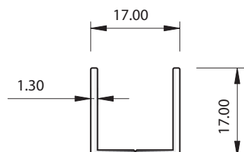
SECTION No. 31017 0.170 kg/m P = 98.88
