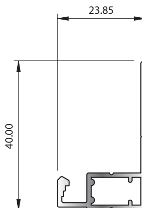
SECTION No. 34918 ACCEPTS STAKING ANGLE X429E 0.325 kg/m P = 143.76
