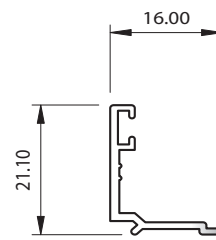
SECTION No. 34733 0.132 kg/m P = 88.11
