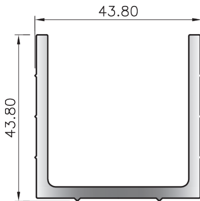
SECTION No. 36089 1.010 kg/m P = 252.82
